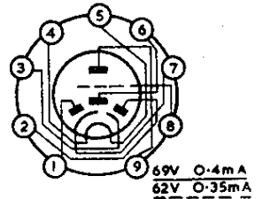
EABC80
