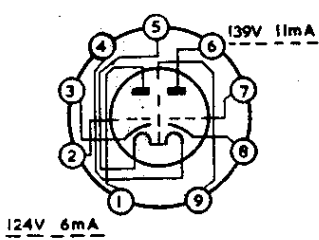
ECC85
